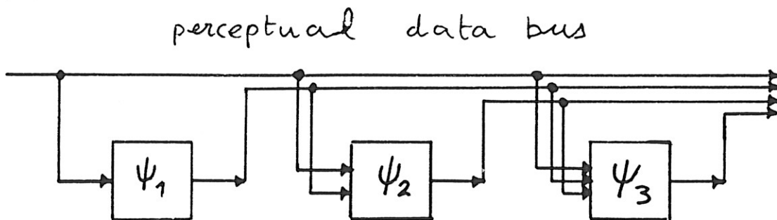
FIGURE 2: (a) Serra's sequential processing scheme. (b) Kent's incremental processing scheme.
